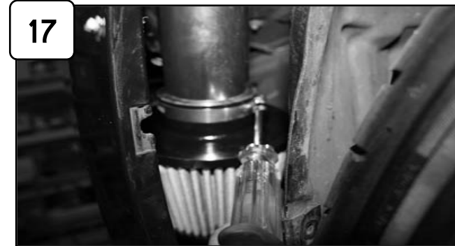
17 Install air filter and tighten using 5/16" nut driver. Attach pre filter to filter if desired. Re-install plastic fender well and re-connect battery terminals.
