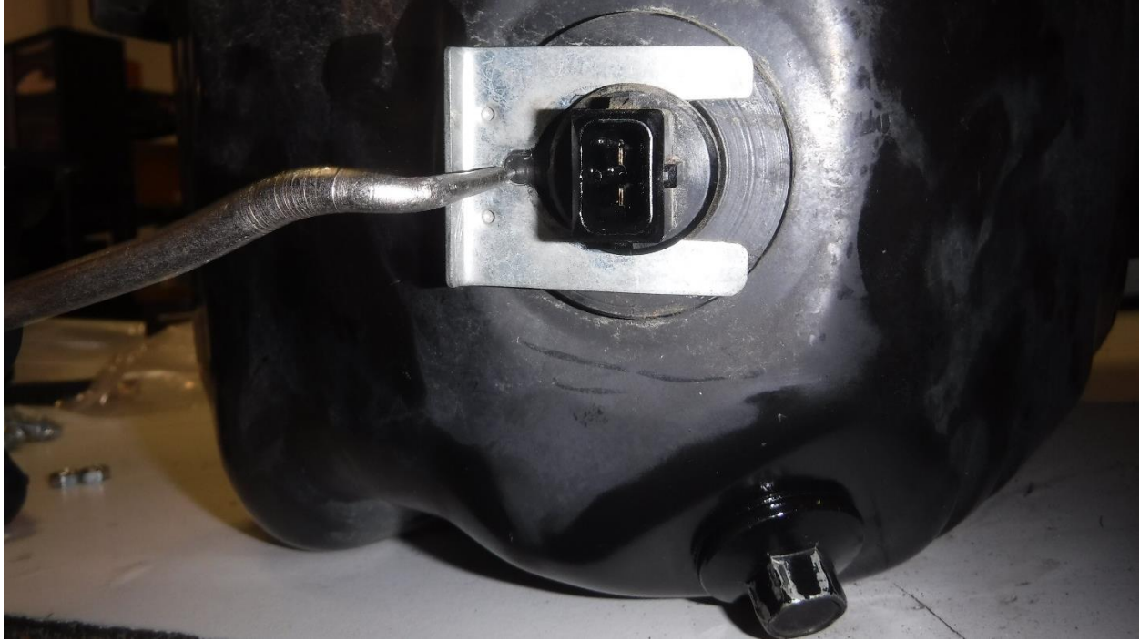
13. Pry the metal holding clip from the outside of the oil pan.
