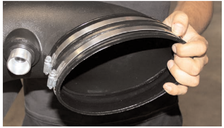
13- Position coupling onto intake tube with supplied clamps. Do not fully tighten.
