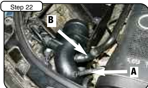
Install provided 3"L x 3/8"D hose with 3/8" elbow onto forth from bottom fitting. Install factory elbow onto last fitting, use provided clamp to tighten down to factory metal tube.
